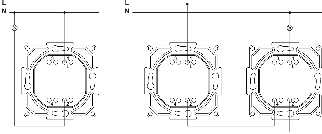
Anahtar
