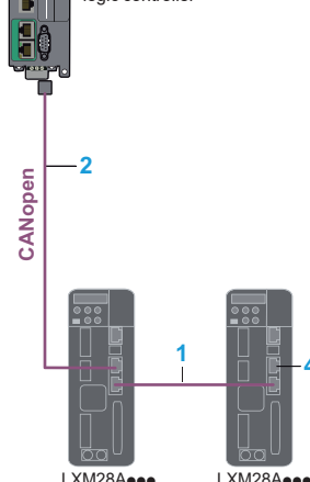
Examples of architectures with control by Modicon M241/M251 logic controllers or LMC058 motion controller
