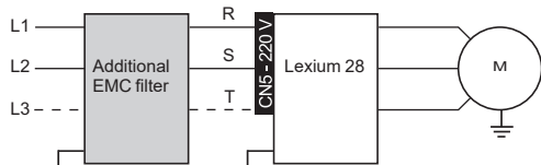
Lexium 28 servo drive with additional EMC filter
