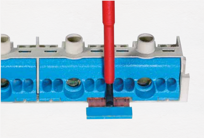
Pluggable jumpers for different N potentials
